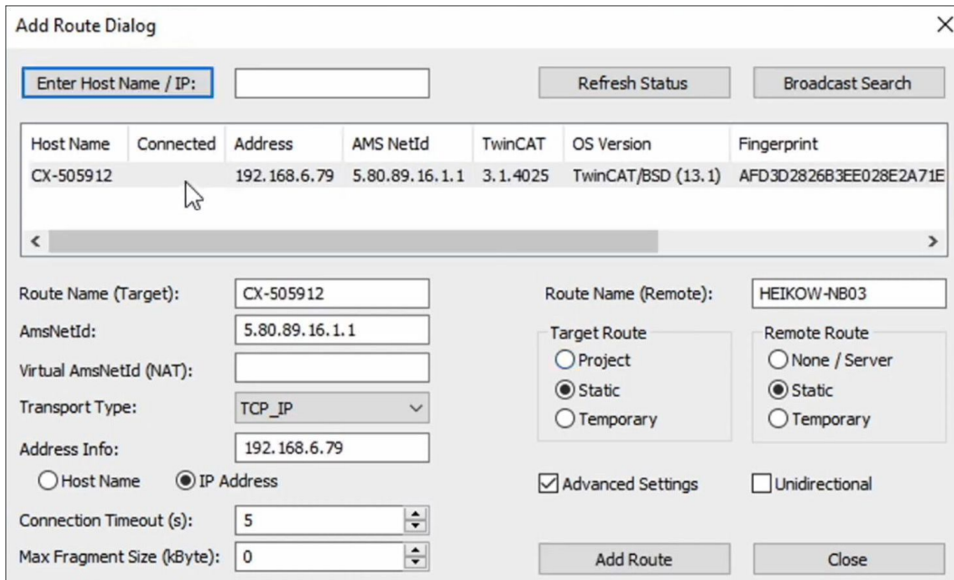
Fig. 2: Add-Route dialog with a TwinCAT/BSD target system and associated IP address.
