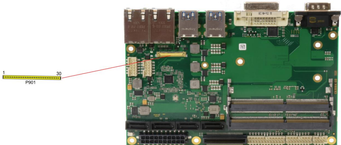
Pinout 30pin connector DVI/HDMI/DisplayPort:
