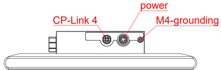
bottom view
