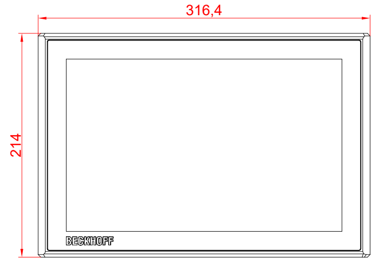
front view
