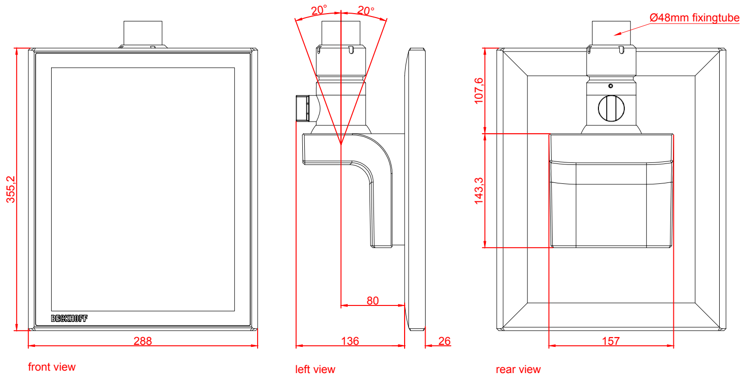
left view
