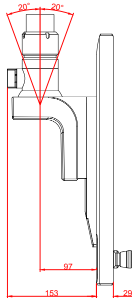
left view
