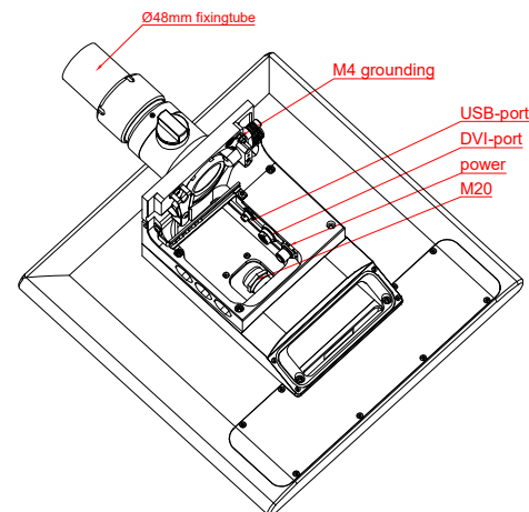
rear view
