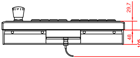
left view
