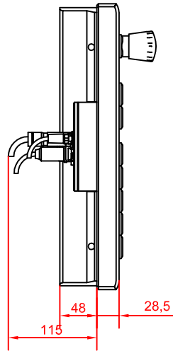
left view
