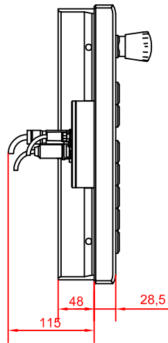
left view
