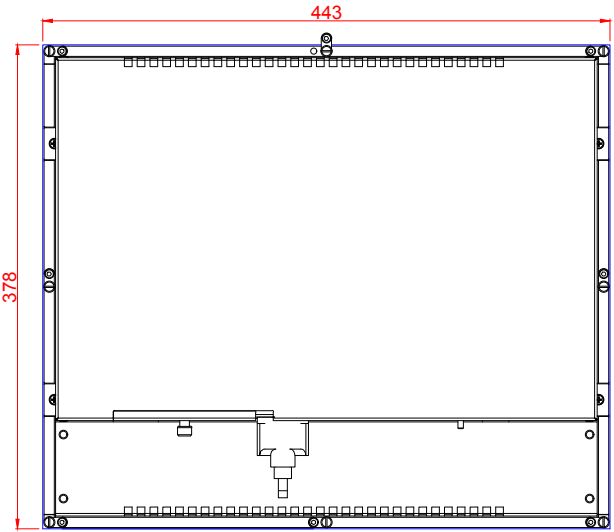
cut out dimensions: 378mm x 443mm
