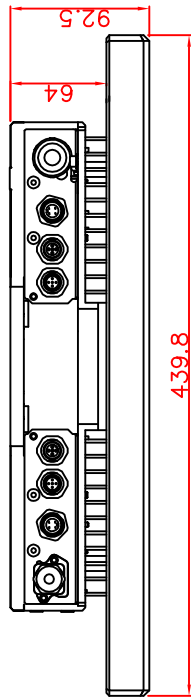
bottom view
