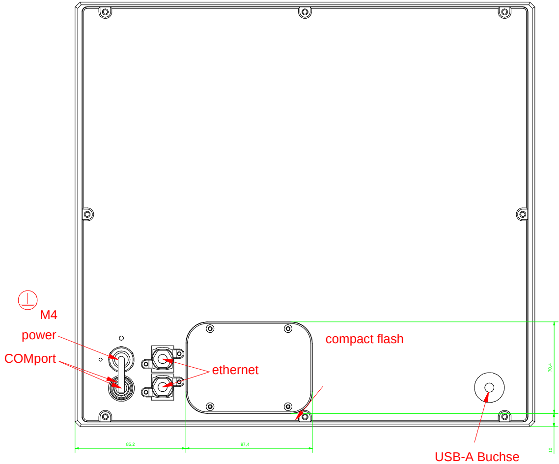
rear view
